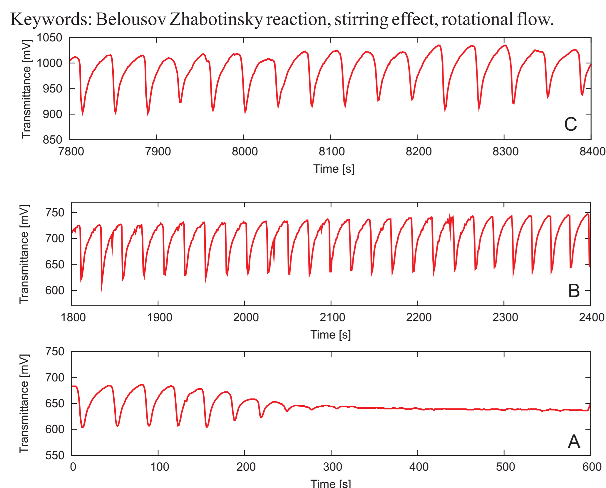
Figure 2: Color oscillations in different phases of the reaction: A: Oscillations in the initial unstirred phase (from time 0s to 600s). B: Oscillations within the stirring phase (from time 1800s to 2400s) and C: oscillations in the unstirred phase C (from time 7800s to 8400s)
